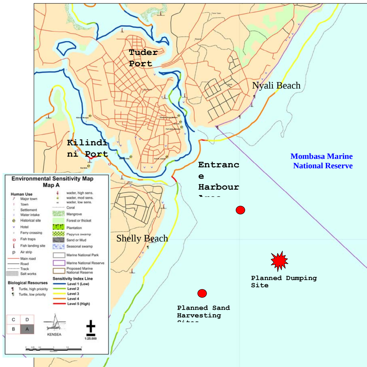
Figure 8.5 Environmental Sensitivity Map of the Mombasa Port entrance area, showing also the sites of the proposed sand harvesting and planned dumping (modified after KenSea; Tytsen 2006)
