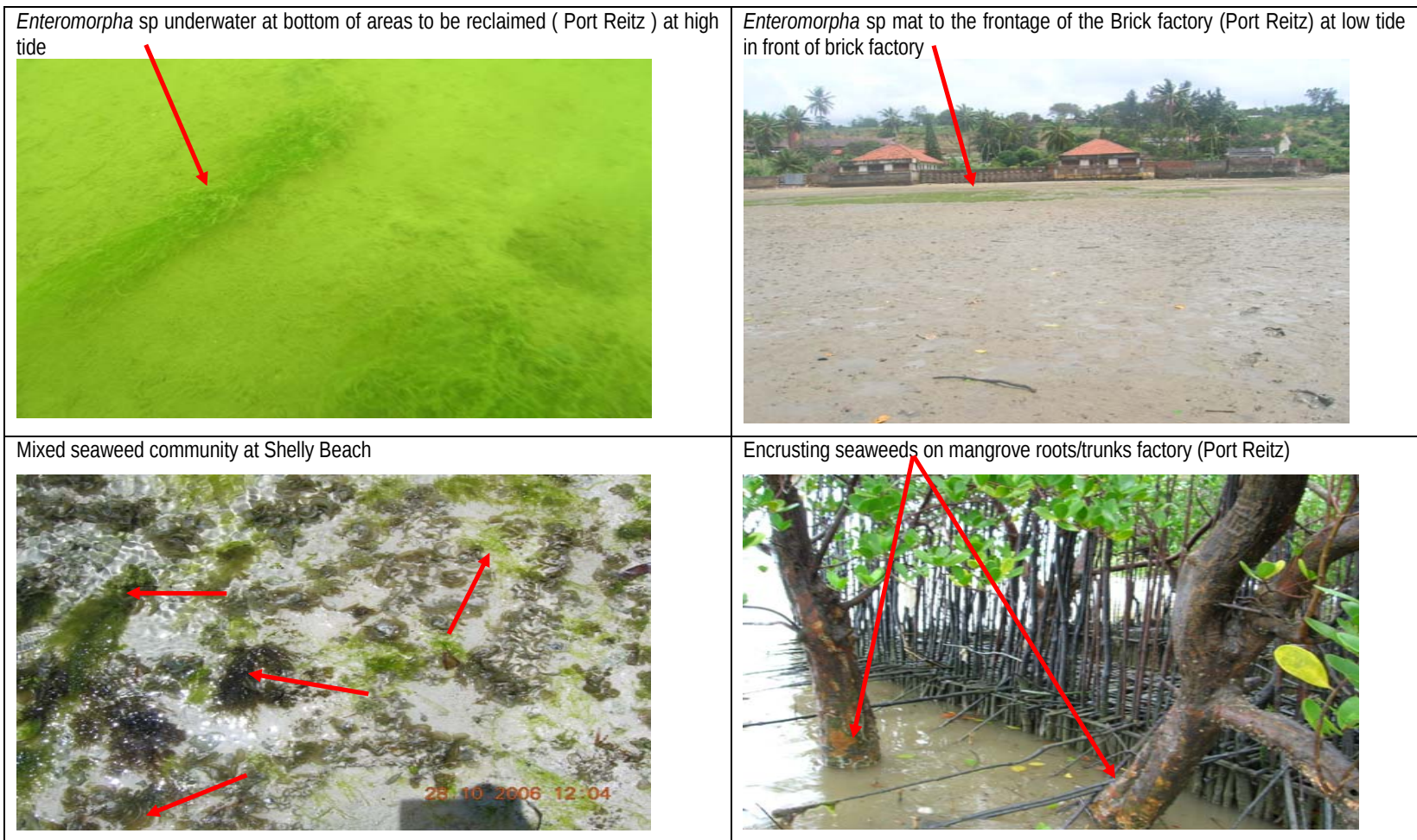
Figure 8.11: Types of seaweed community assemblages found in the Port Reitz creek & Shelly Beach
